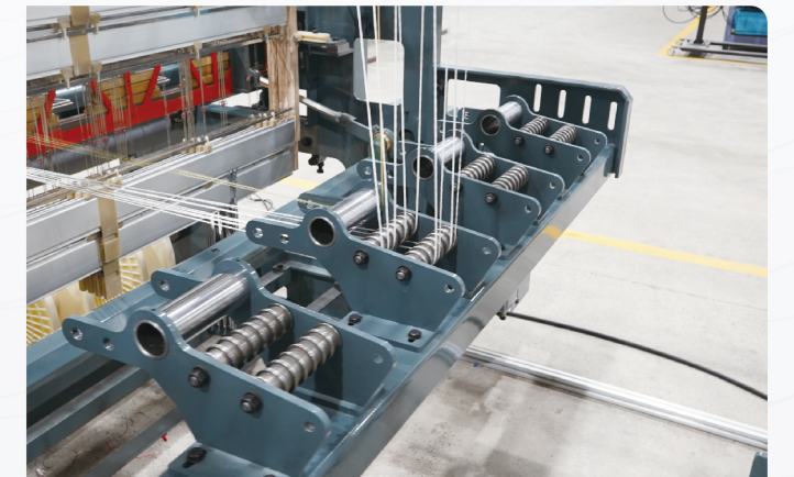
Warp points with guide wheels Layer system
