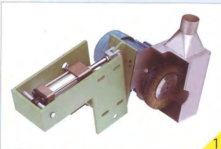
针板清理装置 Pin plate cleaning device
