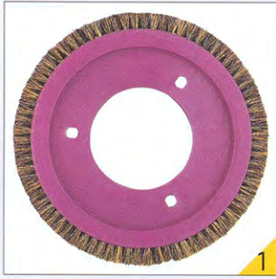
力根毛刷轮 (LK) φ 200 × φ 80 × 20
