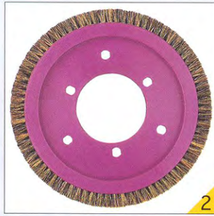
力根毛刷轮 (LK) φ 200 × φ 70 × 20
