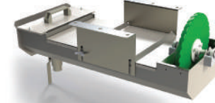
10 EF-GLU/H Gum Application Unit (Horizontal Chain Rails)
