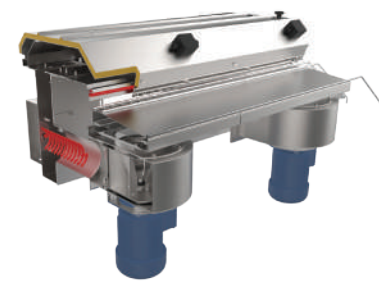
11 EF-EDU/IR Edge Drying Unit (With Infrared & Air Blowers)
