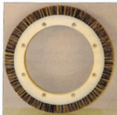
Reggianni brushing ring 240 mm diameter
