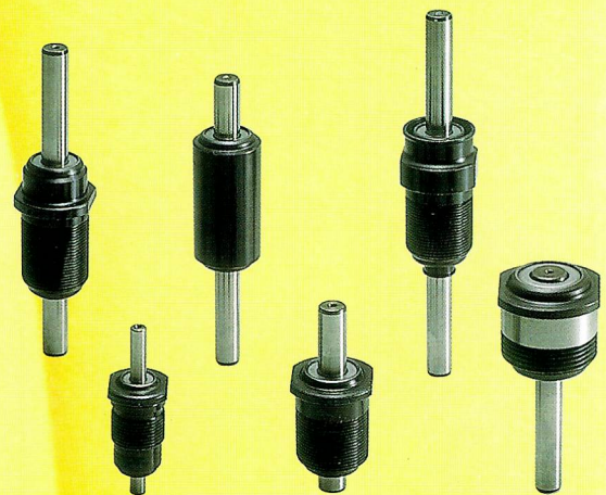
AWA False Twist Spindles (Indirect-Drive Spinners, Over-Drive Type)
