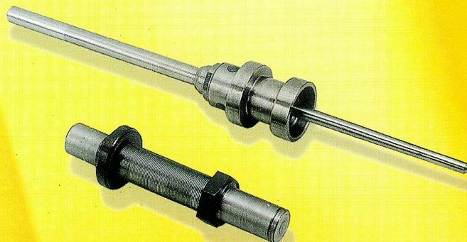
Draw Twister & Bolster (for HZ-68 & HD-68C)
